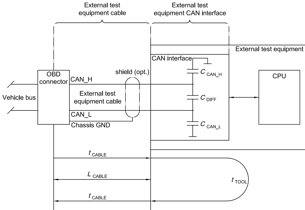
Figure 8 — External test equipment electrical parameters
